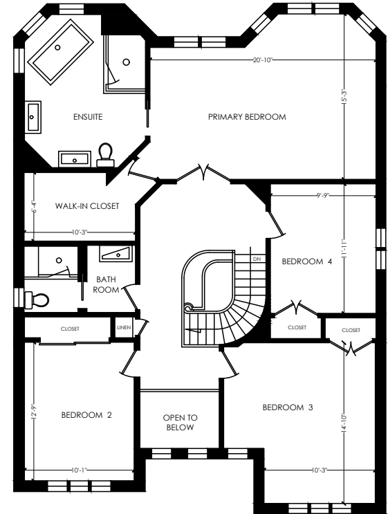
SECOND FLOOR FLOOR AREA 1489 SQ.FT.
