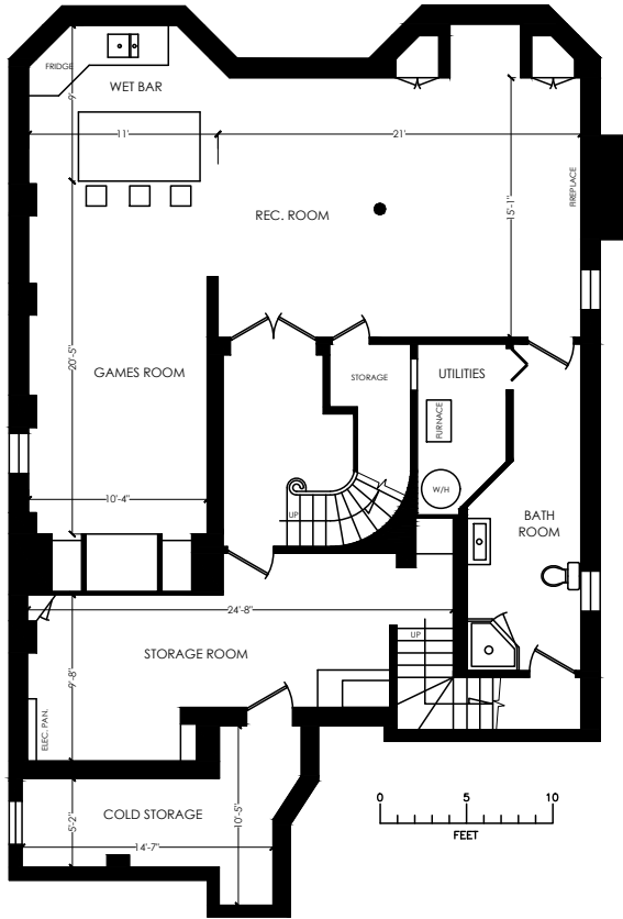
BASEMENT FLOOR AREA 1442 SQ.FT.
