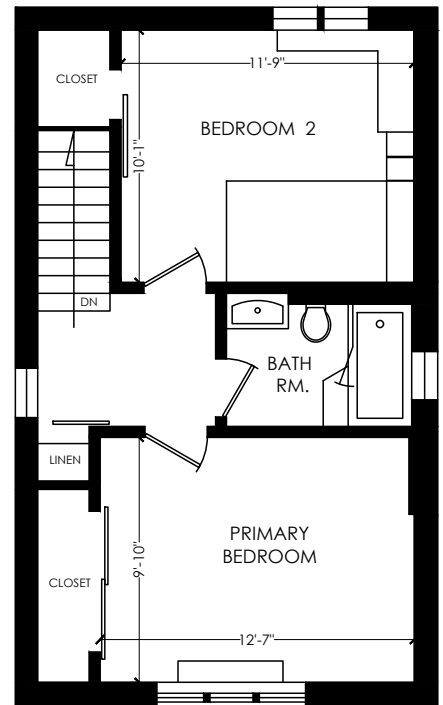
SECOND FLOOR FLOOR AREA 474 SQ.FT.
