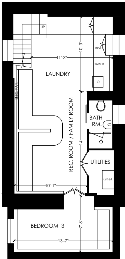
BASEMENT FLOOR AREA 585 SQ.FT.
